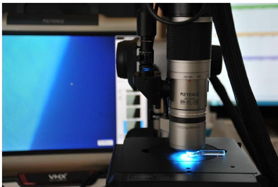
Figure 6. An example setup of digital microscopy measurement in cross-sectional view.
