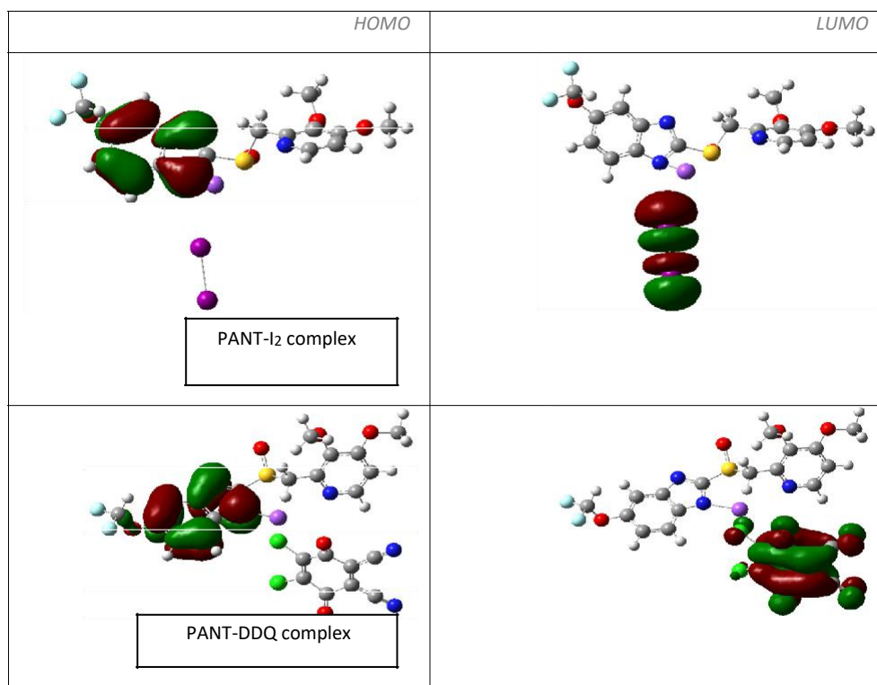
Figure 5. The structures of donor and acceptors by using Gaussian computational chemistry.
