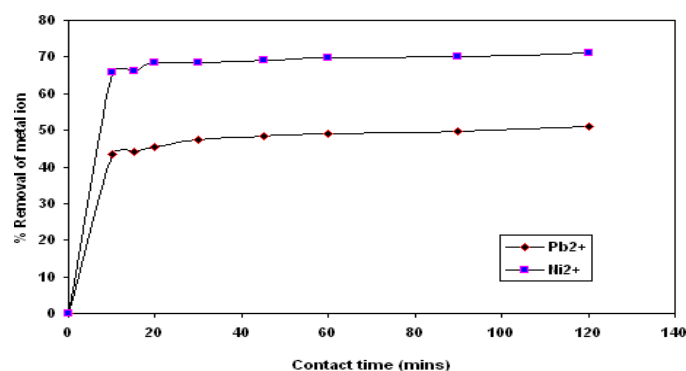
Figure 5. % Removal of Pb^{2+} and Ni^{2+} Vs Contact time for 0.5MOPF adsorbent.
