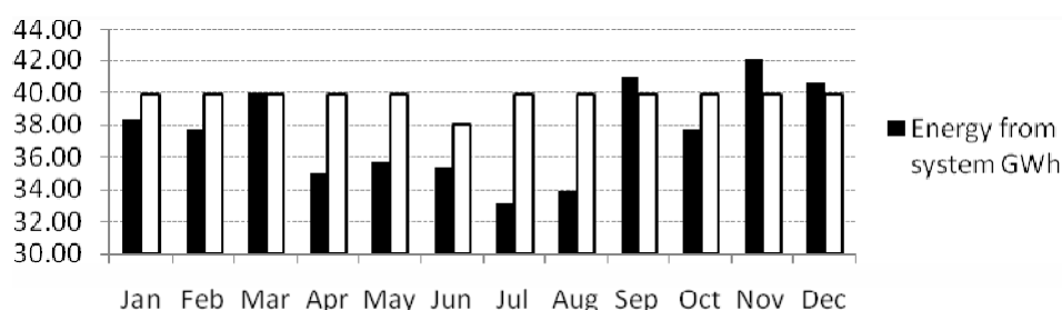
Figure 4a. Comparison of recorded system energy and simulated energy.
