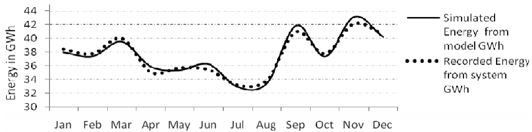
Figure 3b. Model fitting using recorded data of energy production.
