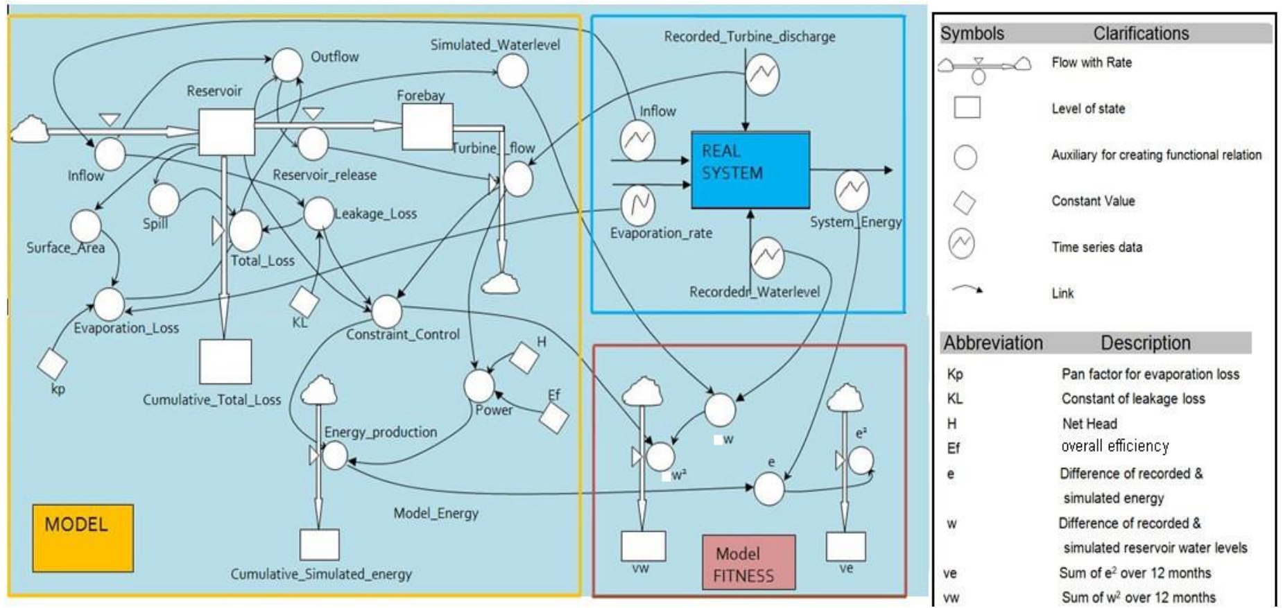
Figure 2. Powersim diagram of Melka Wakena Hydropower Plant System.
