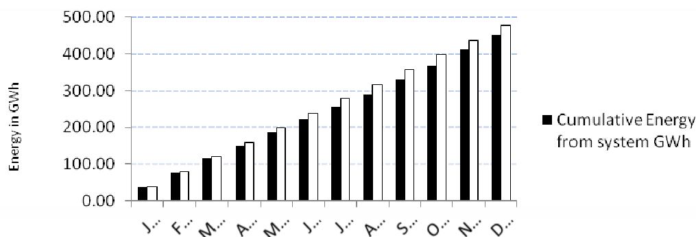
Figure 4b. Comparison of system energy and simulated energy.
