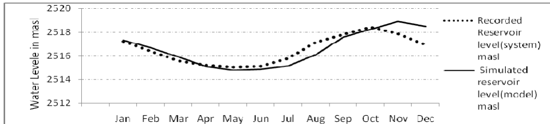
Figure 3a. Model fitting using data of recorded water elevation.
