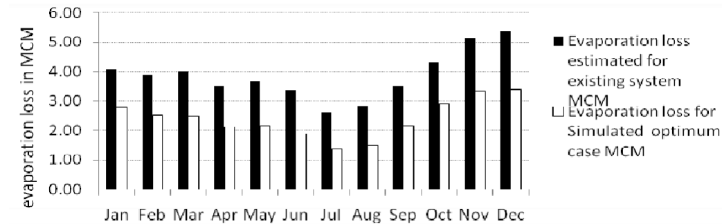
Figure 5. Comparison of estimated monthly evaporation losses.
