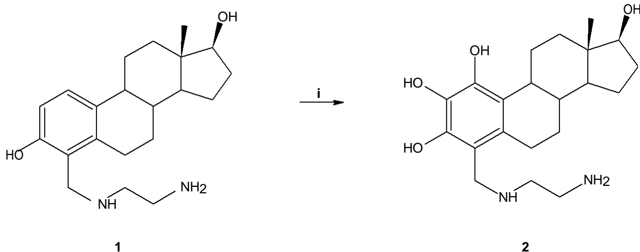
Figure 1. Synthesis of 4-[(2-Amino-ethylemino)-methyl]13-methyl-7,8,9,11,12,13,14,15,16,17-decahydro-6H-cyclopenta[a]-phenanthrene-1,2,3,17-tetraol (2); ii) \text{Cl}_2/\text{AlCl}_3 , \text{H}^+ .
