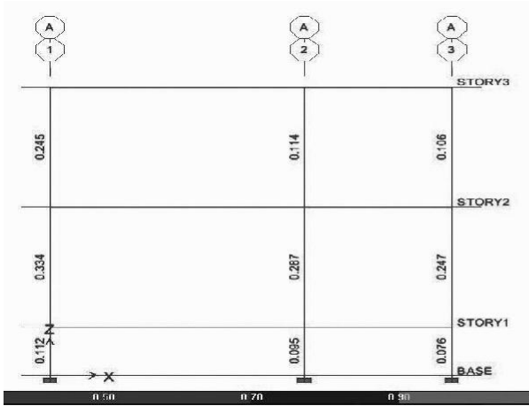
Figure 7. Section from Column's internal forces in the double story sample building.
