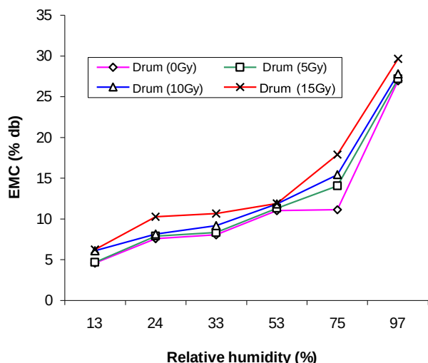
Figure 5. Water absorption isotherm of irradiated and non-irradiated Drum cowpea stored at 27°C.
