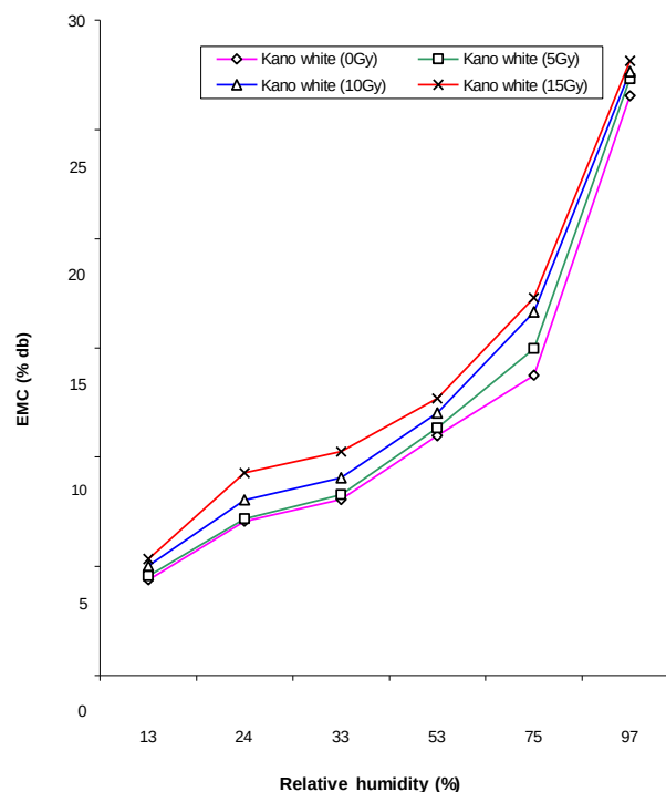
Figure 4. Water absorption isotherm of irradiated and non-irradiated Kano white cowpea stored at 18°C.
