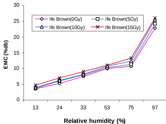
Figure 1. Water absorption isotherm of irradiated and non-irradiated Ife brown cowpea stored at 27°C.
