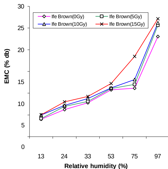
Figure 2. Water absorption isotherm of irradiated and non-irradiated Ife brown cowpea stored at 18°C.
