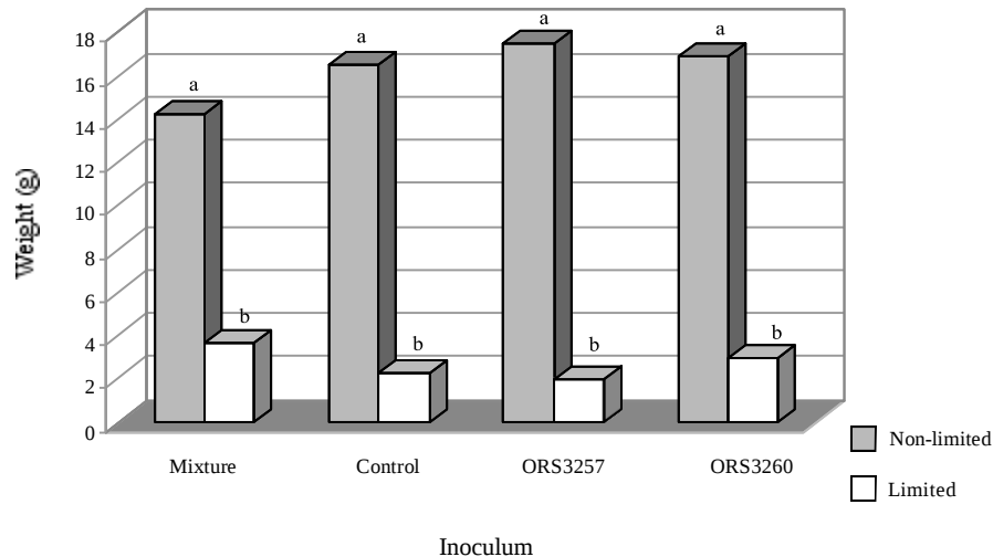
Figure 6. Water regime effect on reproductive part dry weight of plants inoculated with different inoculums. Values for each water regime followed by the same letter are not significantly different at P < 0.05 (Tukey test).
