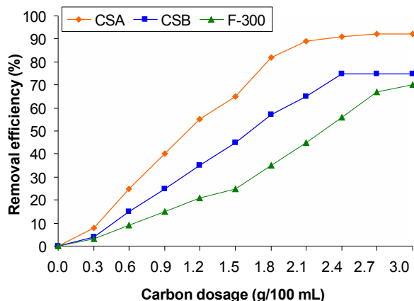
Figure 1. Removal efficiency of COD by the activated carbons.
