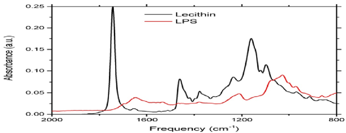
Figure 4. FTIR spectra of pure lecithin and LPS.
