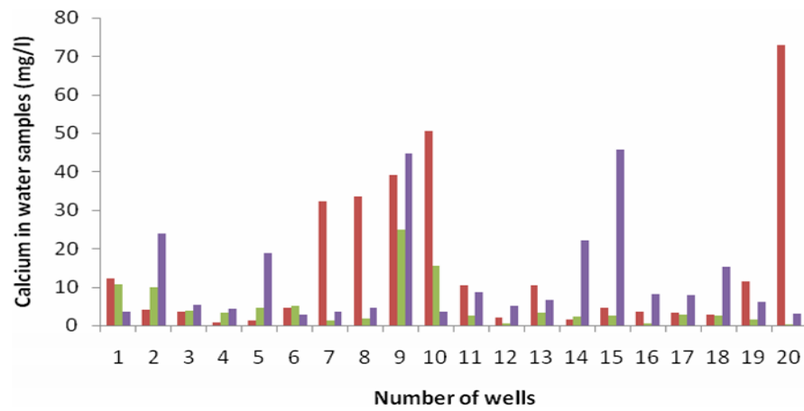
Figure 8. Calcium in water samples of Ifo, Ibogun and Pakoto.
