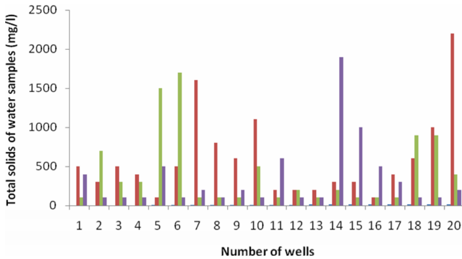
Figure 2. Total solids of water samples in Ifo, Ibogun and Pakoto.
