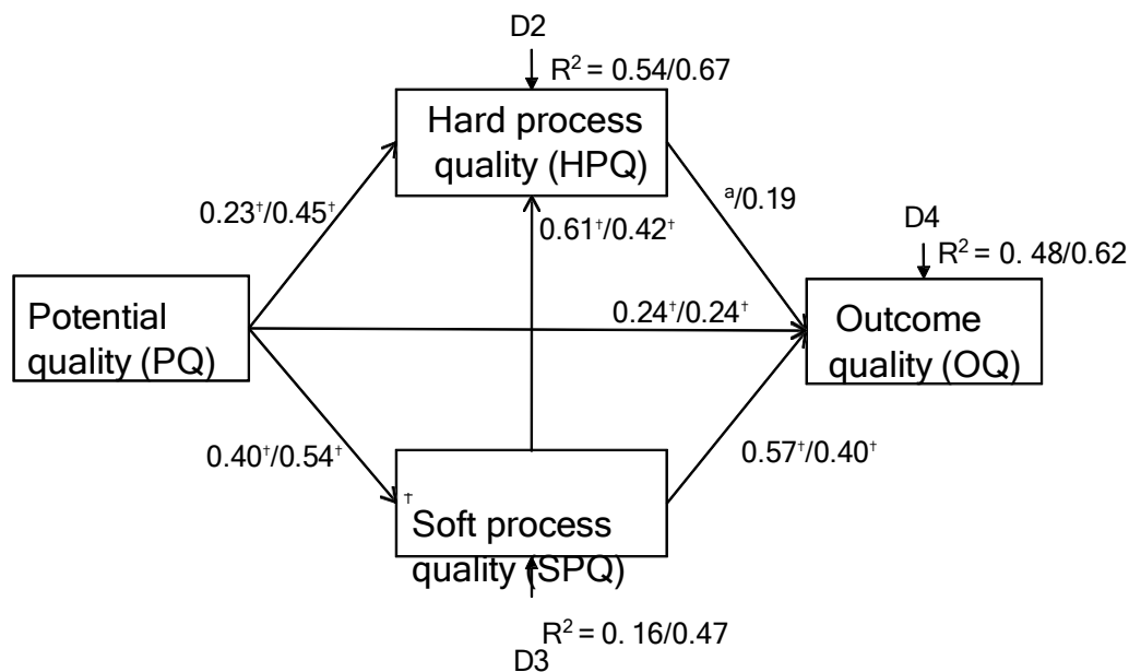
Figure 4. Path comparisons of models based on Gounaris (2005c) and Study 2 data. † = p < .01 . All coefficients are standardized. Gounaris (2005c) coefficients are before slash, while Study 2 coefficients are after slash. a For Gounaris (2005c) model, this coefficient is very close to zero with a large residual, and is therefore removed to enable over-identification.
