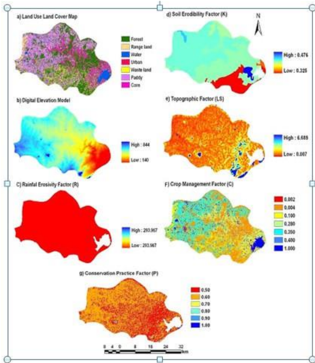
Figure 1. Thematic layers of USLE factors.
