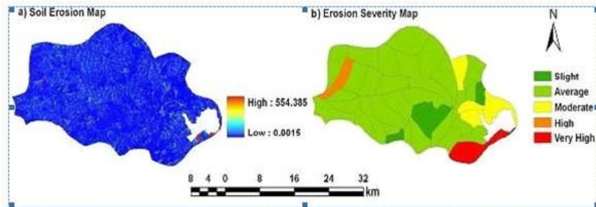
Figure 2. Soil erosion map and micro watershed wise severity map.
