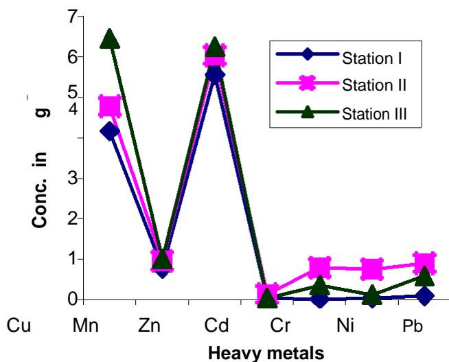
Figure 5. Annual mean concentrations of heavy metals in Chrysichthys nigrodigitatus at the three stations.
