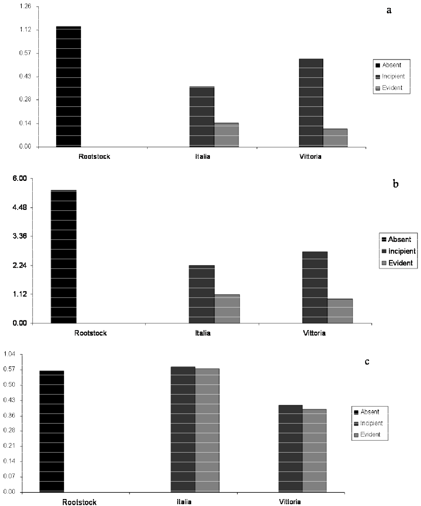
Figure 3. Ratios between the active forms of selected cations, \text{Fe}^{2+}/\text{Cu}^{2+} (a), \text{Fe}^{2+}/\text{Mn}^{2+} (b), \text{K}^+/\text{Ca}^{2+} (c) in the rootstock and the variously stressed scions.
