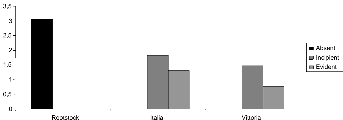
Figure 2. Total chlorophyll content (mg g -1 fm) in unstressed (rootstock) and variously stressed scions.
