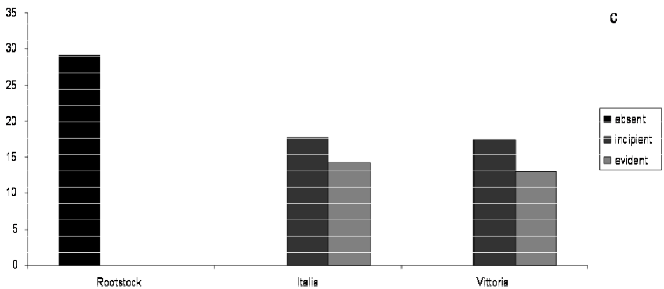
Figure 1. Dry matter (% a), total nitrogen (% dm, b) and total proteins content ( \text{mg g}^{-1} \text{ dm} , c) in unstressed (rootstock) and variously stressed scions.
